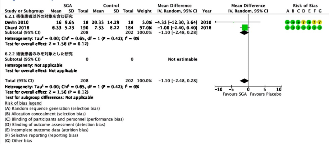
Caption Forest plot of comparison: 3 ICU滞在期間, outcome: 3.2 ICU滞在期間.
